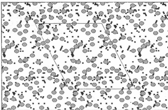
above transition ( T = 318.3 K, f = 0.91 )
