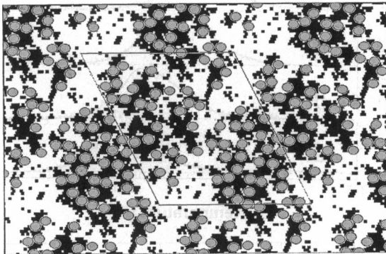
in transition range ( T = 312.55 K, f = 0.52 )
