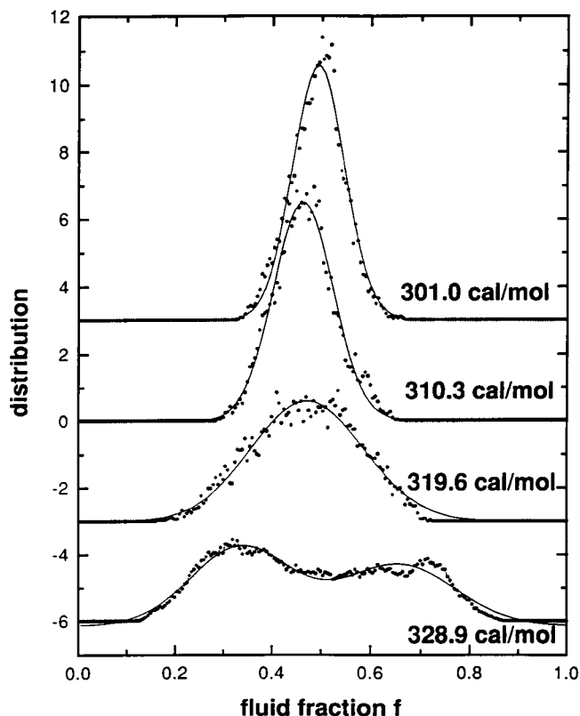
FIGURE 3 Distribution of states during a Monte Carlo simulation at the heat capacity maximum, from top to bottom with \Delta\omega_{gl} = 301.0 , 310.3, 319.6, and 328.9 cal/mol. All other parameters as in Fig. 2. The bottom curve has more than one maximum, indicative of a first-order transition. All other curves represent second order transitions (see text). Solid curves are fits with one-component or two-component (bottom) Gaussian distributions.
