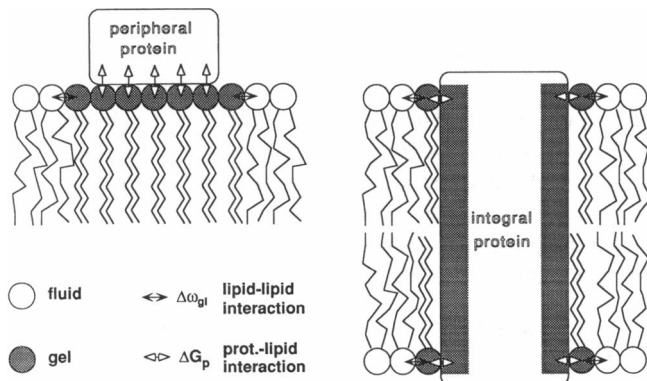
FIGURE 1 Schematic picture of lipid-protein association. Local interactions \Delta\omega_{gl} and \Delta G_p for peripheral (left) and integral proteins (right) are indicated with solid and open arrows, respectively.
